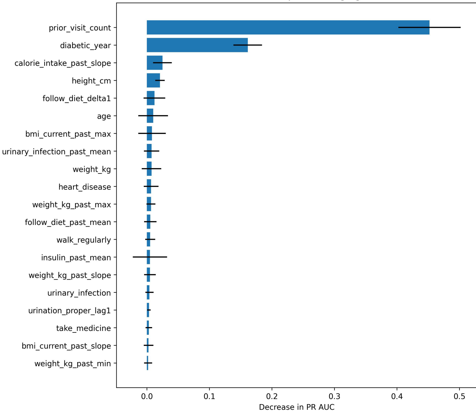
Permutation importance: lightgbm
